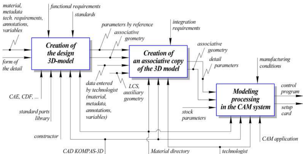
F i g. 3. Diagram of the process of transferring part parameters from the design model to the CAM system
