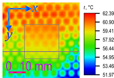
Figure 3. Thermogram of the defective region and its surroundings. The defective area is shown by a dotted square; the selected section is shown by a line
