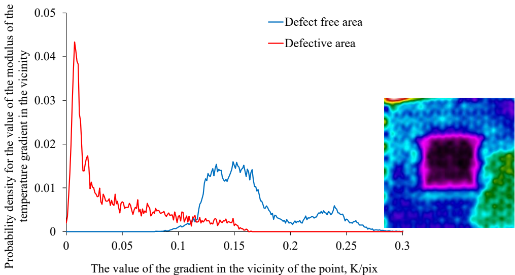
Fig. 11. Distribution of the values of the informative parameter of the improved method in the defective region and its surroundings
