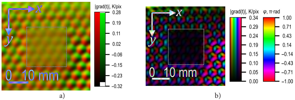
Figure 2. Distribution of gradients in the defective area and its surroundings: a) in rectangular coordinates, the red component is x , the green component is y ; b) in polar coordinates, color saturation is the value, color tone is the direction; the defective area is shown by a dotted square
