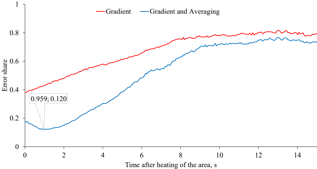
Fig. 10. Error proportion before and after improving the method by introducing averaging
